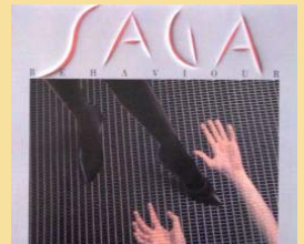
SAGA: Behaviour
